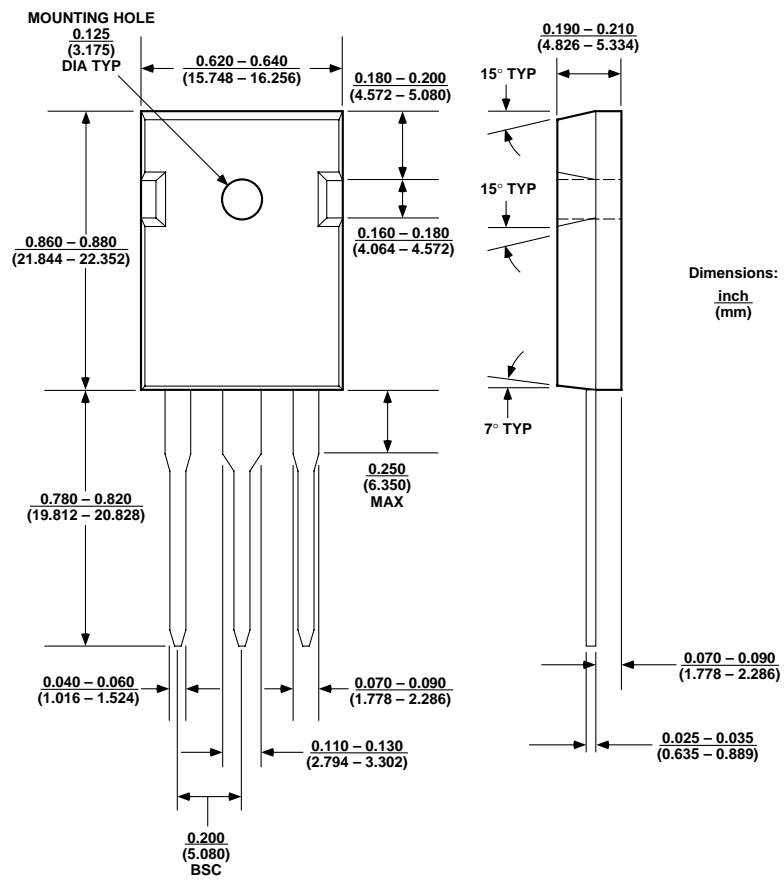
3-Lead TO-247 (WT)
