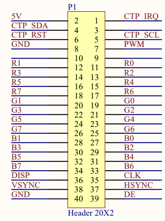
RGB Header Interface
