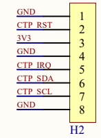
Touch Panel interface
