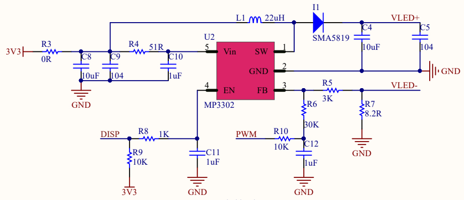
LCD Backlight Power
