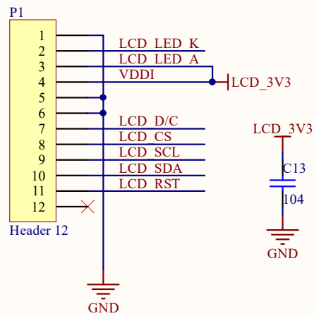
LCD Interface
