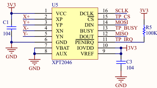
Touch Screen
