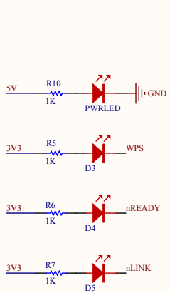
LED
