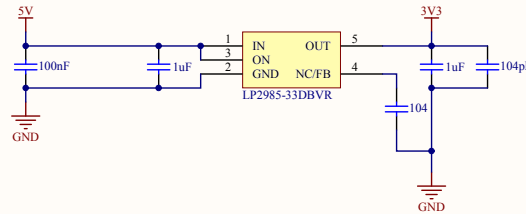
Power Supply
