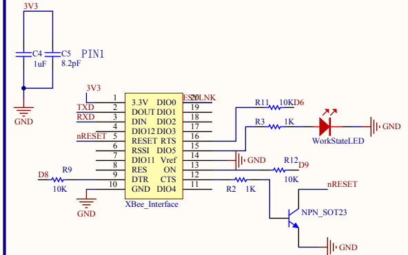
XBee_Interface
